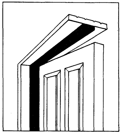
In door trim, Stop is nailed to the faces of the door frame to prevent the door from swinging through. As window trim, Stop holds the bottom sash of a double-hung window in place. Also used as an apron under window stools.
