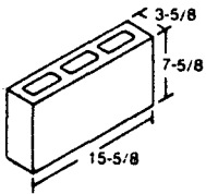
4 x 8 x 16 STRETCHER SKU NO. 301035
