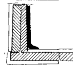
SET-ON BASE For use with hard surface floors.
