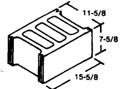
12 x 8 x 16 STRETCHER SKU NO. 301055
