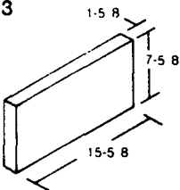
2 x 8 x 16 SOLID SKU NO. 301059
