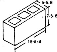
6 x 8 x 16 STRETCHER SKU NO. 301040
