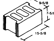
10 x 8 x 16 STRETCHER SKU NO. 301050
