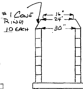
30" CATCH BASIN 7 BLOCKS PER RING
