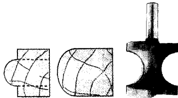
BULL NOSE BIT 2 FLUTE
