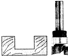
STRAIGHT 2 FLUTE
