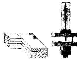
REVERSIBLE TONGUE & GROOVE ASSEMBLY 2 WING
