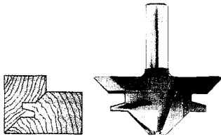
LOCK MITER
