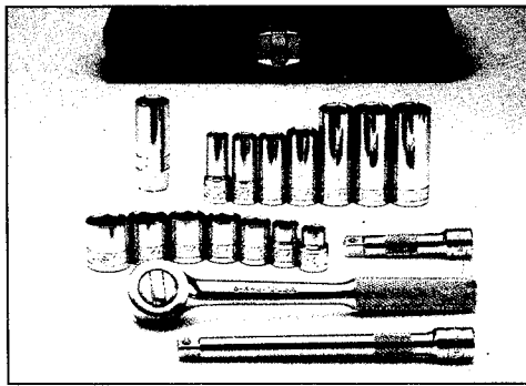
Fractional Socket Set SKU NO. 710026, MFG. NO. 94520 18-piece 3/8" drive. Sizes, Standard: 3/8", 7/16", 1/2", 9/16", 5/8", 11/16", 3/4". Deep: 3/8", 7/16", 1/2", 9/16", 5/8", 11/16", 3/4", 5/8" spark plug socket. 7 1/2" ratchet. 3" ext.. 6" ext.. metal box.
