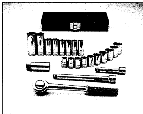
Metric Socket Set SKU NO. 710022, MFG. NO. 91820 22-piece 3/8" std. metric drive: sizes 10, 11, 12, 13, 14, 15, 16, 17, 18, 19MM. Deep sockets, 10, 11, 12, 13, 14, 15, 17, 19MM. 5/8" spark plug socket, 7 1/2" ratchet. 3" ext., 6" ext., metal box.
