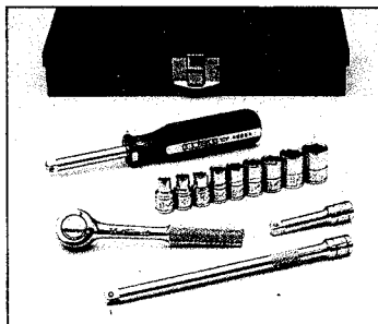
Fractional Socket Set SKU NO. 702394 MFG. NO. 4913 13-piece 1/4" std. Drive: sizes 3/16", 7/32", 1/4", 9/32", 5/16", 11/32", 3/8", 7/16", 1/2", 4 1/2" ratchet. 6" spinner handle, 2" ext., 6" ext., metal box.
